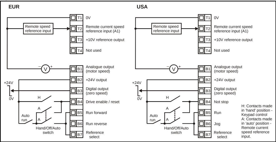
Figure 10-35 Pr 11.27 = HUAC
