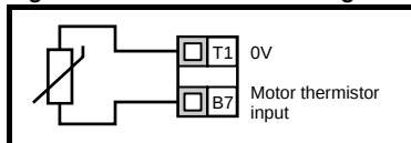
Figure 10-22 Connection diagram
