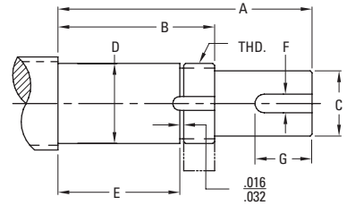
TYPE 3C1, REQUIRED FOR QUICK MOUNT BEARING
