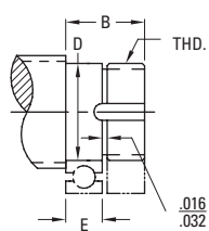
TYPE 1A1, REQUIRED FOR FLOATING BEARING
