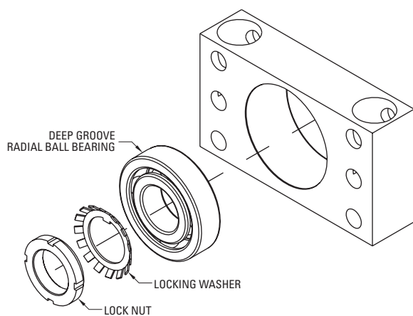
Floating Bearing Support (1)(2)
