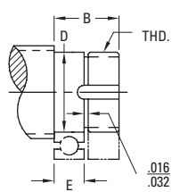
TYPE 1A1, REQUIRED FOR FLOATING BEARING
