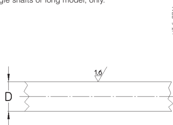
b) Albero macchina passante b) Machine passing through shaft
